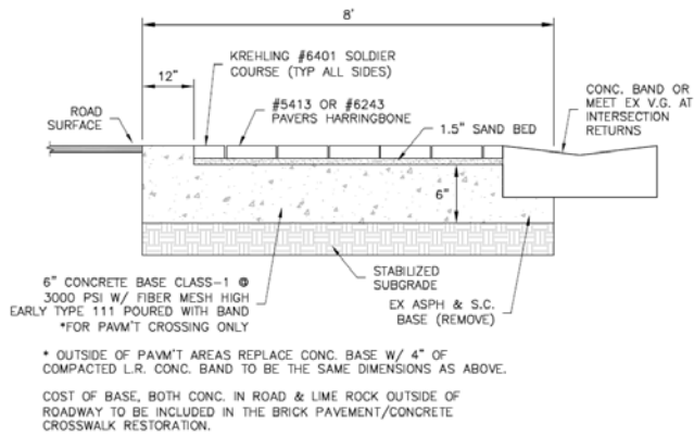
PAVER BLOCK CROSSWALK DETAIL NTS
